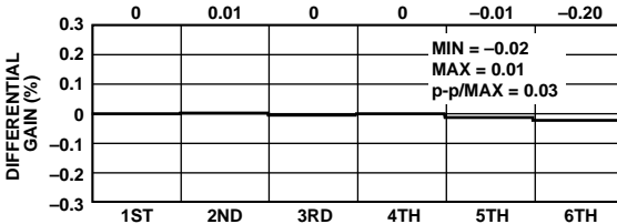
Figure 3. Typical Composite Output Differential Gain and Phase, NTSC for X Channel; f = 3.58 MHz, R_L = 150 \Omega
